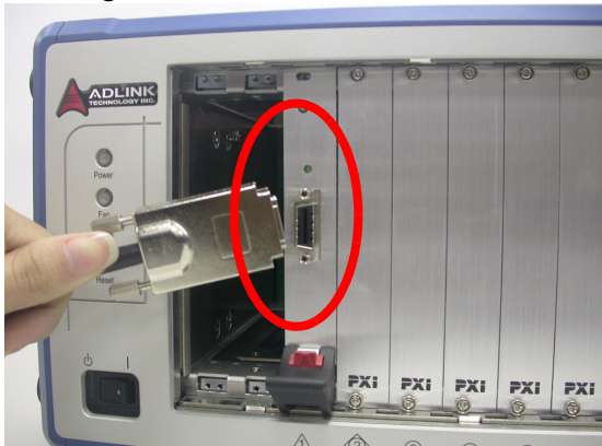
Figure 2-6: Laptop Computer Connected to a PXI™ Extension Chassis
