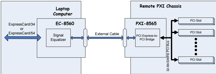
Figure 3-1: PCI Express-to-PXI Extension Kit Functional Block Diagram
