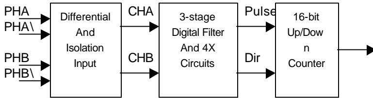
Fig 5.1 Encoder Interface Block Diagram
