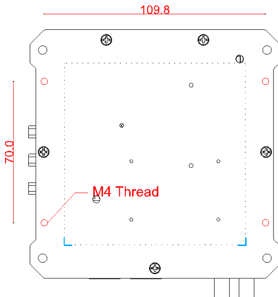
Screw hole locations/ measurements, and thermal pad position (dotted lines)
