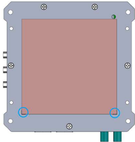
For the optional thermal pad (90x90x0.5mm), attach it by aligning it with the indicated corners in blue
